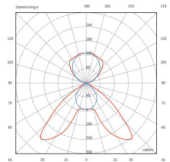
SERIES 5506 T5 2x54W PENDANT
